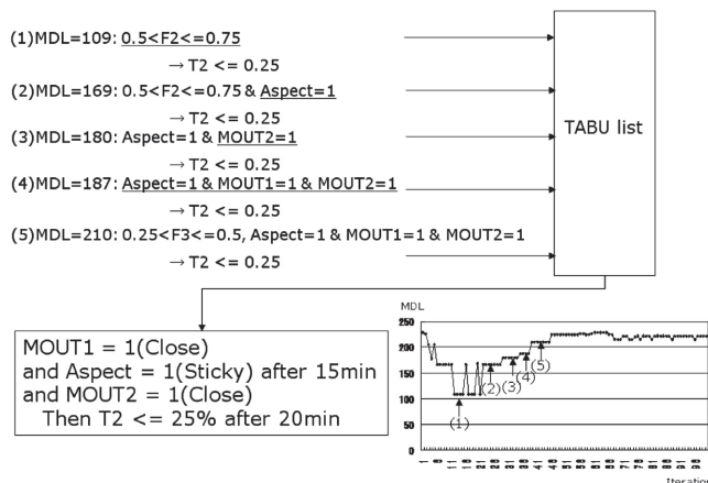
Fig.7 The Experiment of Tabu Learning Classifier System
