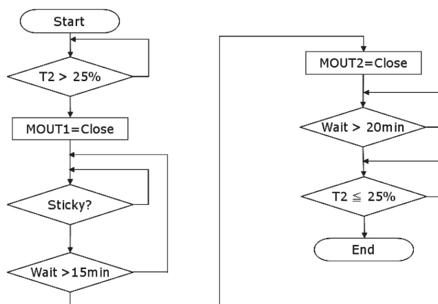
Fig.8 The Extracted Workflow of Experts
