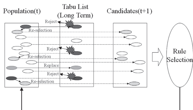
Fig.6 Tabu Learning Classifier System
