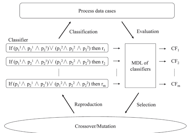
Fig.2 Learning Classifier System
